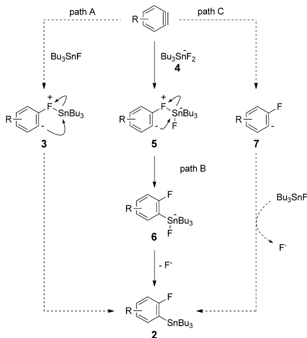
Scheme 3. Plausible pathways for the fluorostannylation.
