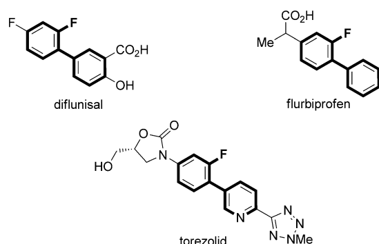
Scheme 1. Representative biologically active compounds containing a 2-fluorobiaryl motif.
