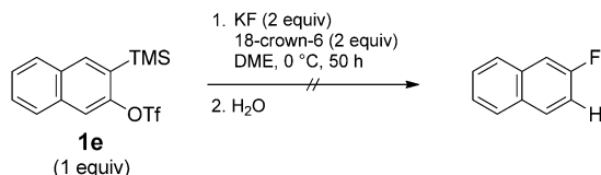
Scheme 5. Reaction of 2,3-naphthalene with a fluoride ion.
