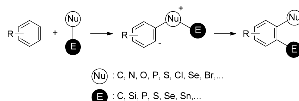
Scheme 2. Insertion of arynes into \sigma bonds between a nucleophile and an electrophile. Nu = nucleophile, E = electrophile.
