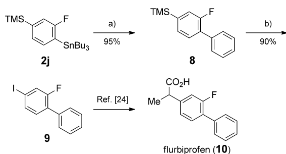
Scheme 6. Formal total synthesis of flurbiprofen: a) 2j (1 equiv), iodobenzene (1 equiv), [Pd(dba) 2 ] (10 mol%), PPh 3 (40 mol%), CuI (75 mol%), DMF, 50 °C, 21 h. b) 8 (1 equiv), iodine monochloride (2 equiv), CH 2 Cl 2 , 0 °C, 7 h.
