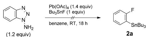
Scheme 4. Reaction of Bu 3 SnF with benzyne generated by oxidation.
